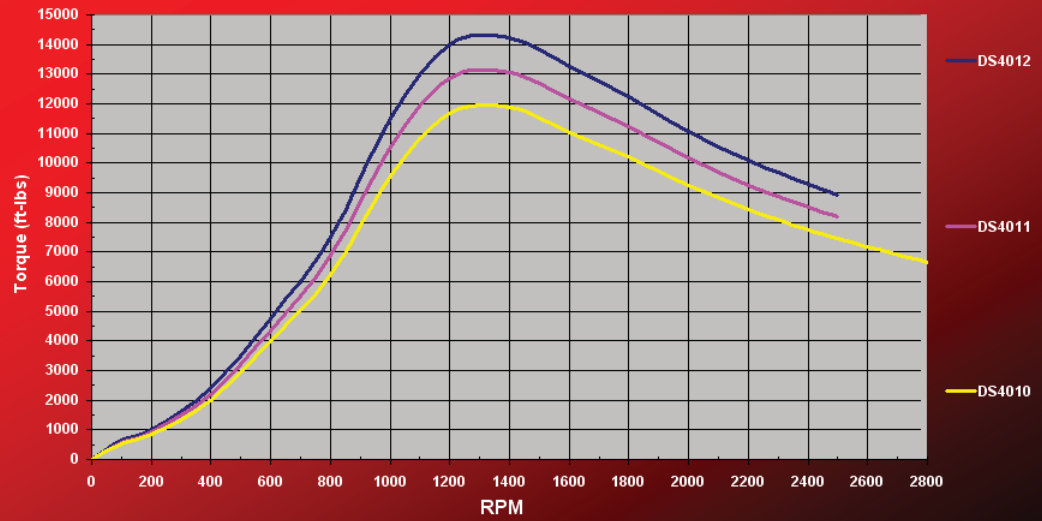
Taylor DS Series Torque Curve, English
