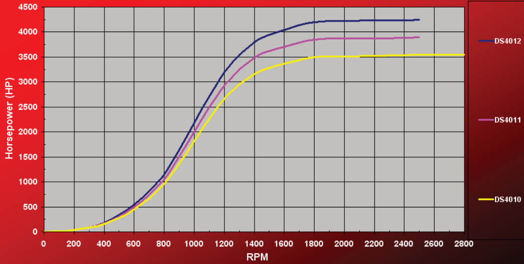
Taylor DS Series Horsepower Curve , English
